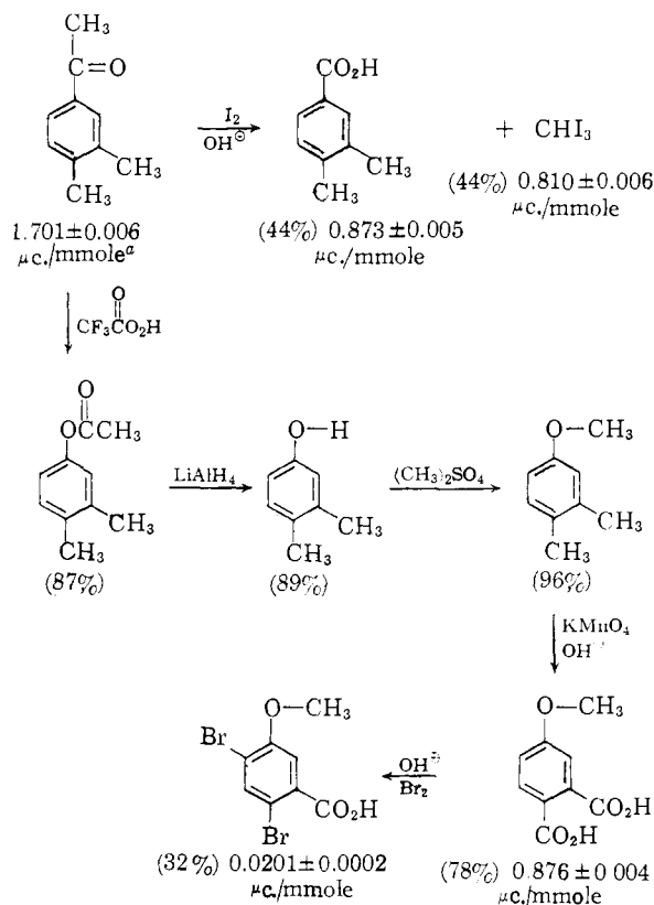
Fig. 2.—Degradation of radioactive 3,4-dimethylacetophenone. Activities are in microcuries per millimole ( \mu\text{c./mmole} ) and were determined by the vibrating-reed electrometer method as described by O. K. Neville, J. Am. Chem. Soc. , 70 , 3499 (1948). Errors are expressed as average deviations in the case of duplicate determinations or as standard deviations when three or more measurements were made (see Experimental). a Measured as the 2,4-dinitrophenylhydrazone; all other compounds whose activities are indicated were assayed directly.
